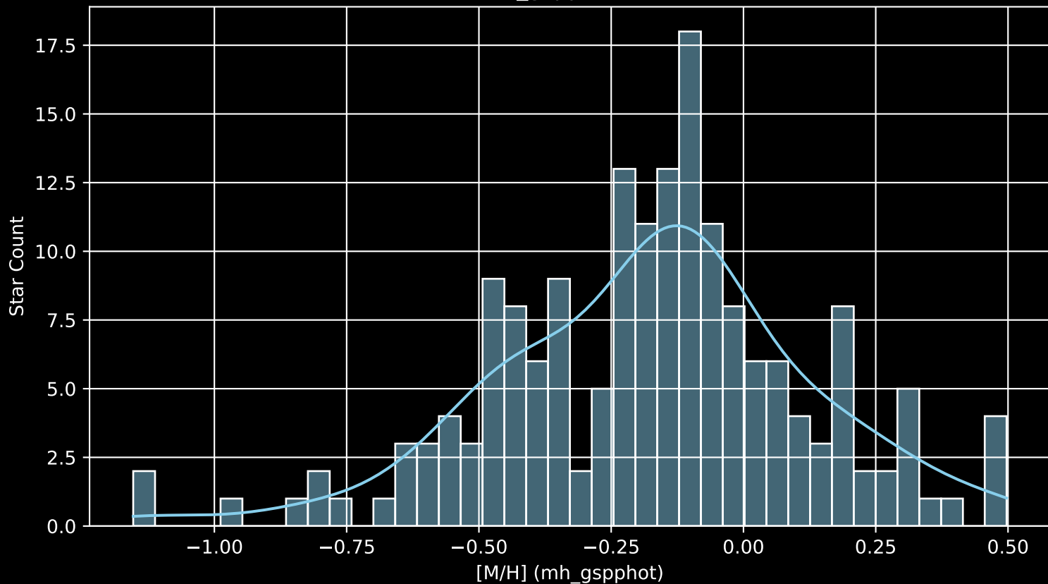
APOGEE DR17 Field: [264+20 [M/H] (mh_gspphot) (n= 176)
