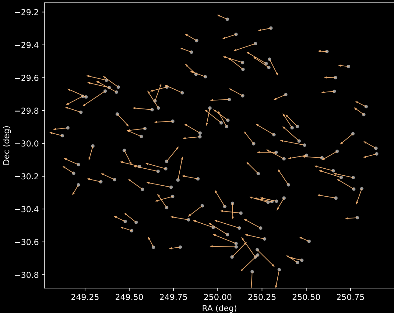
APOGEE DR17 Cluster 3 Proper Motion Vectors (n=117)
