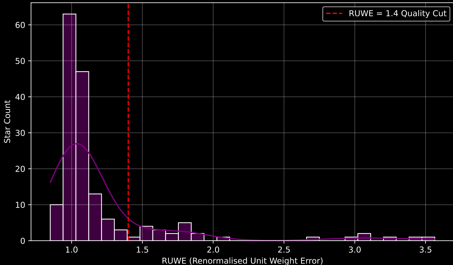
GAPOGEE DR17 Field [264+20] RUWE Distribution (n= 167)
