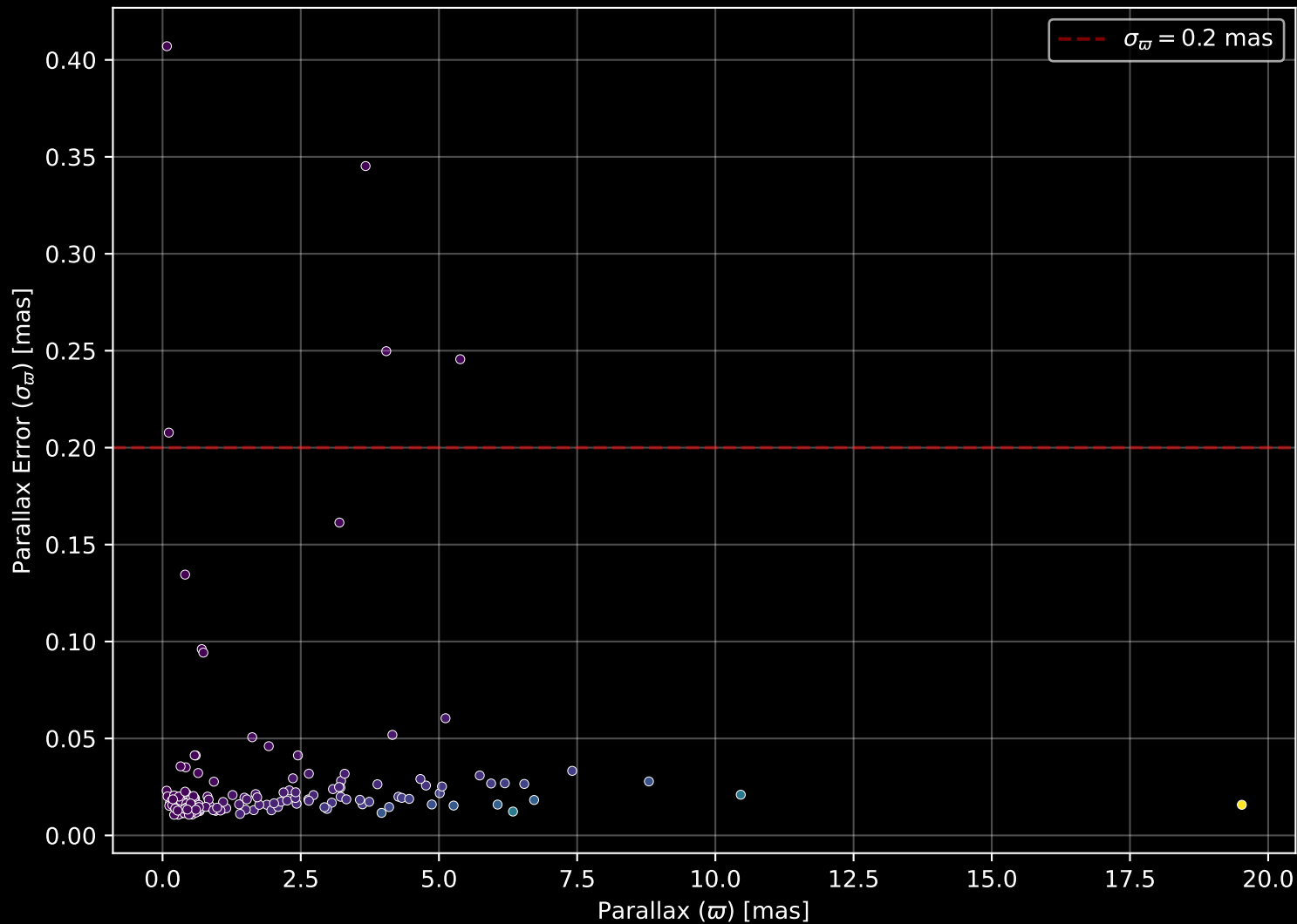
APOGEE DR17 Field: [264+20] Parallax Quality (n= 176)
