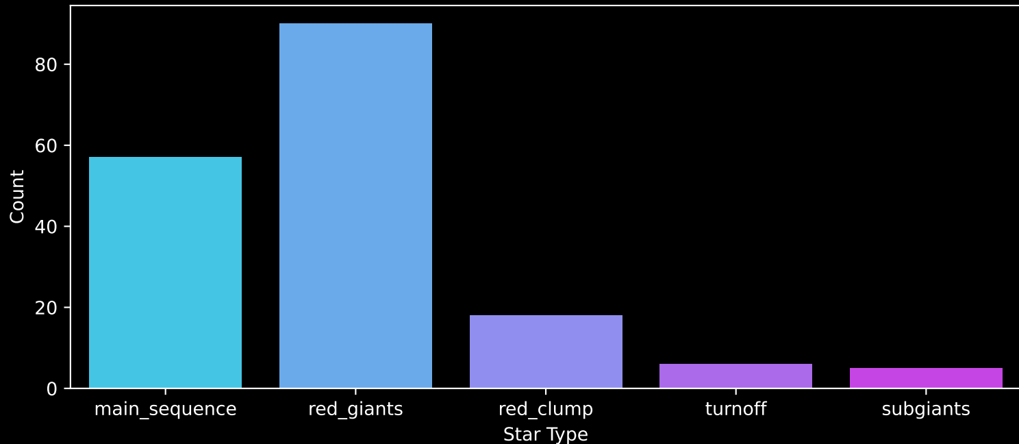
APOGEE DR17 Field: [264+20] Count plot of Star Type
