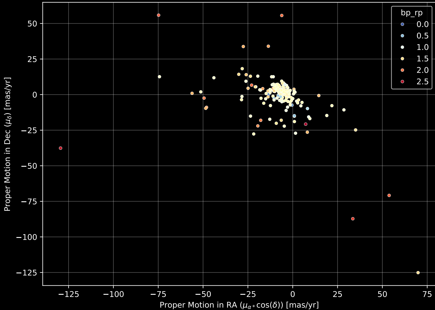
APOGEE DR17 Field: [264+20] Proper Motion Diagram (n= 176)
