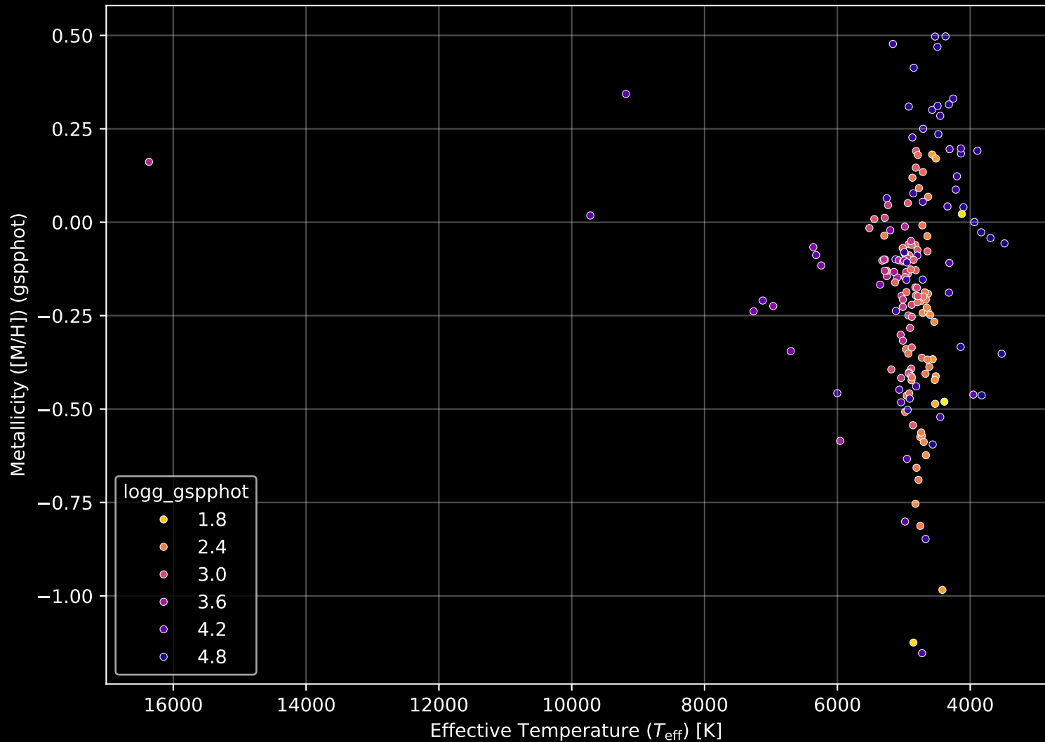
APOGEE DR17 Field: [264+20] Stellar Population Parameters (n= 176)
